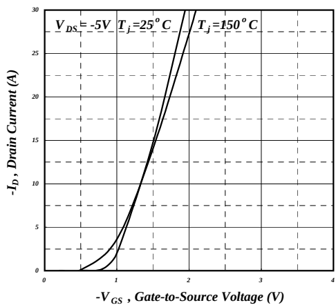
Fig 11. Transfer Characteristics
