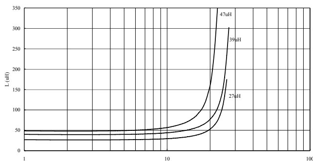
INDUCTANCE vs. FREQUENCY CHARACTERISTICS
