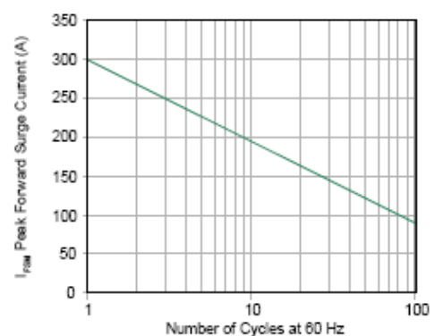
Figure 6 - Maximum Non-Repetitive Peak Forward Surge Current
