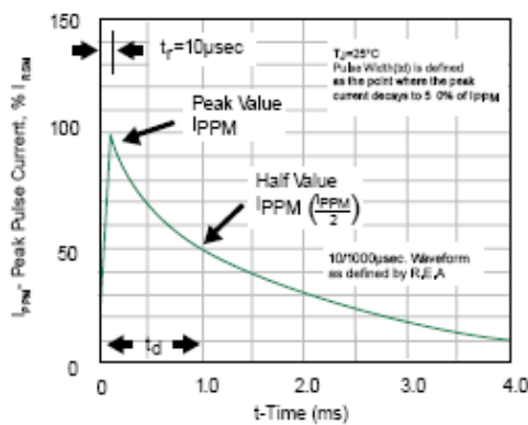
Figure 3 - Pulse Waveform
