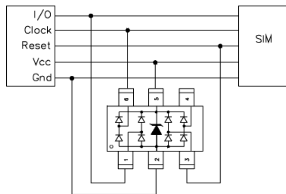
Figure 6 - SIM Port
