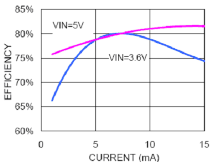
Six LED Efficiency
