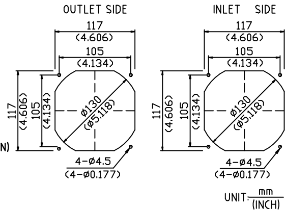
MOUNTING PANEL CUTOUT
