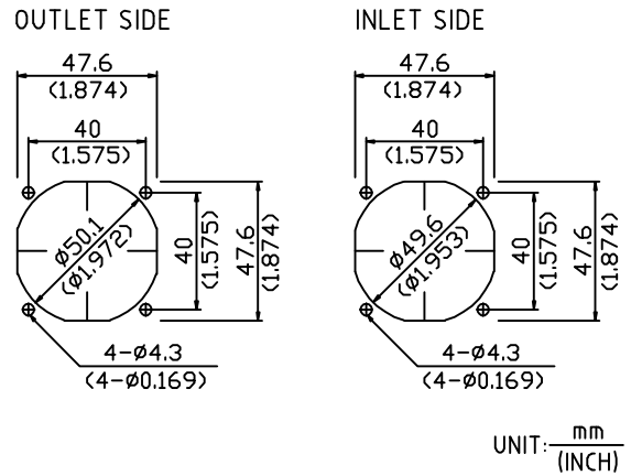
MOUNTING PANEL CUTOUT
