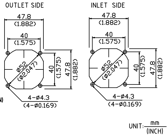
MOUNTING PANNEL CUTOUT
