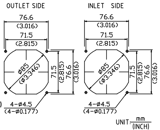
MOUNTING PANEL CUTOUT
