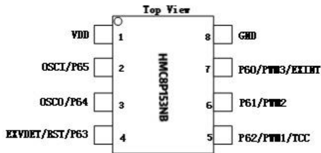
HMC8P153NB-8PIN 脚位图
