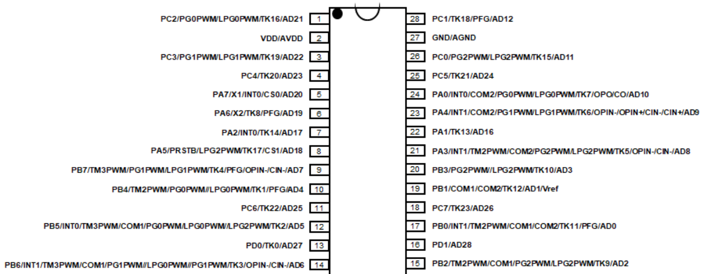
PFC460-S28: SOP28 (300mil) PFC460-T28: TSSOP28
