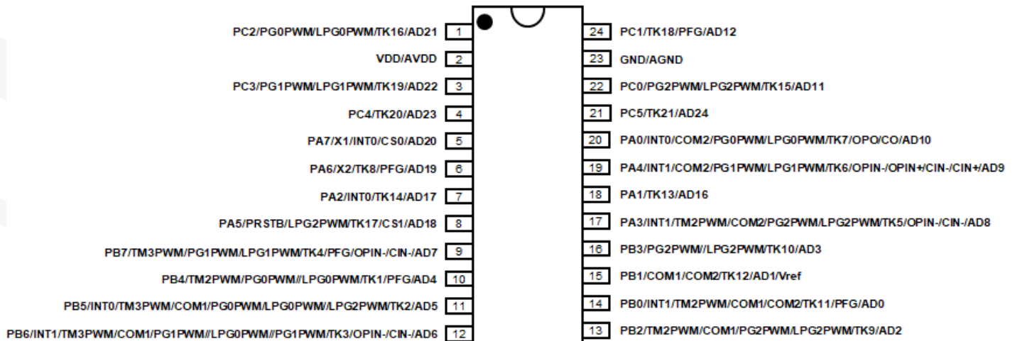
PFC460-S24: SOP24 (300mil)
