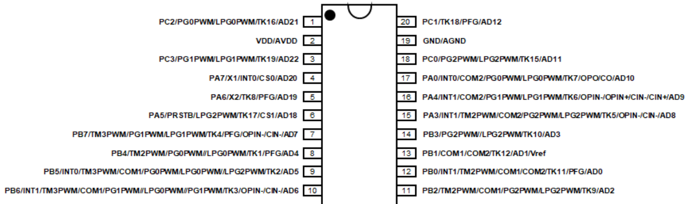
PFC460-S20: SOP20 (300mil) PFC460-H20: HSOP20 (300 mil) PFC460-T20: TSSOP20
