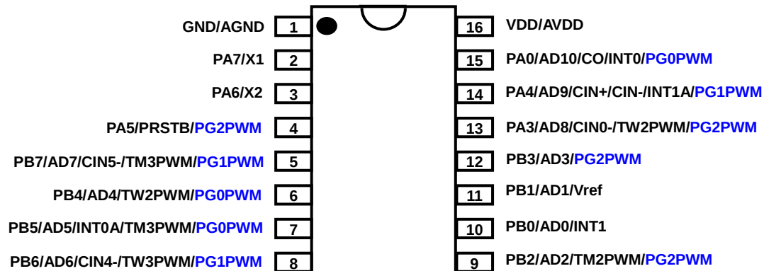
PMS132/PMS132B-S16B (SOP16B-150mil)
