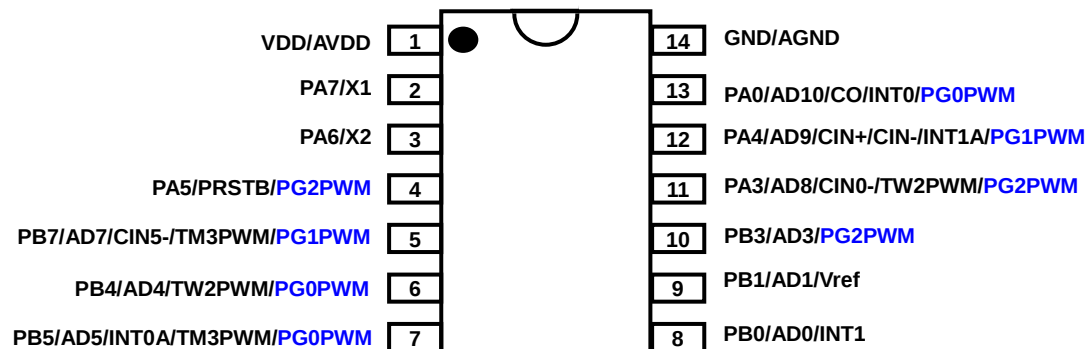
PMS132/PMS132B-S14 (SOP14-150mil)
