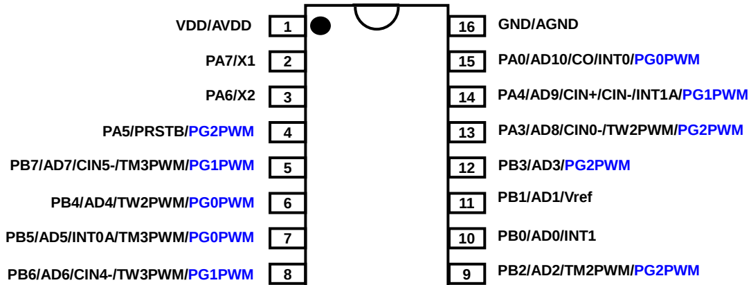
PMS132/PMS132B-S16A (SOP16A-150mil)
