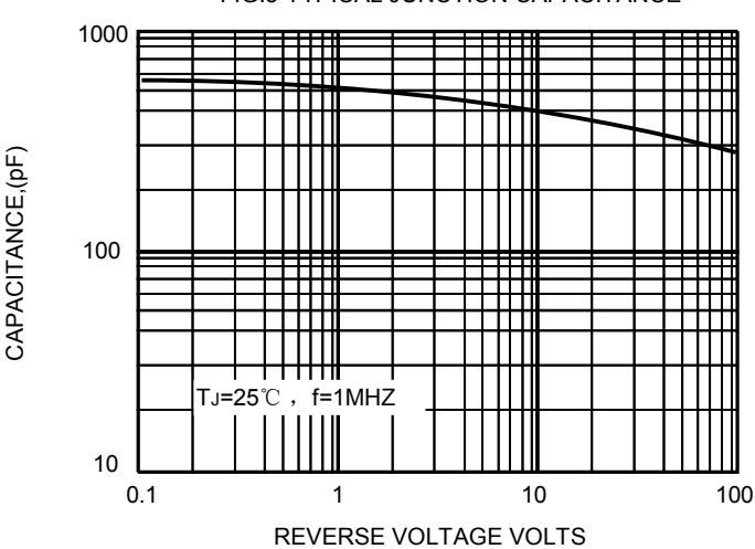
FIG.5-TYPICAL JUNCTION CAPACITANCE
