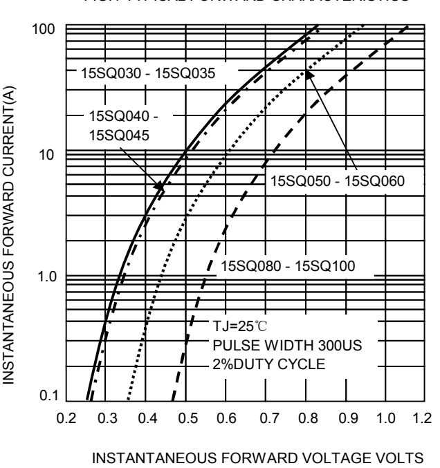
FIG.4-TYPICAL FORWARD CHARACTERISTICS
