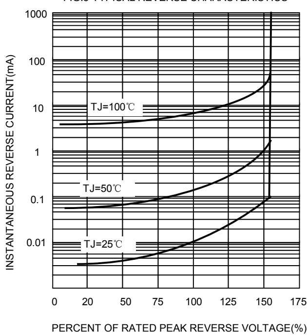
FIG.3-TYPICAL REVERSE CHARACTERISTICS
