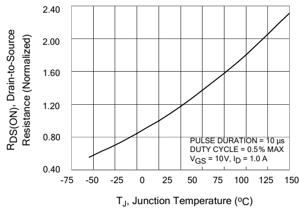
Figure 10. Typical Drain-to-Source ON Resistance
