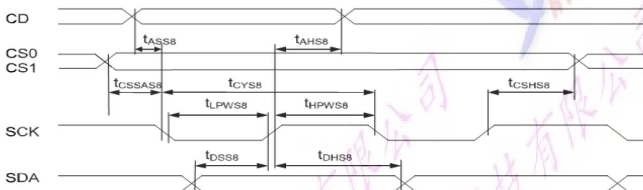
FIGURE 15: Serial Bus Timing Characteristics (for S8 / S8uc)
