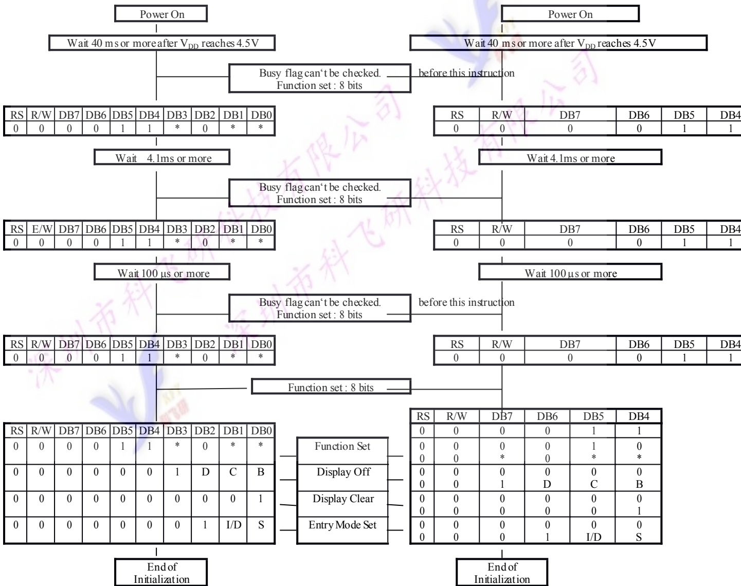
1) 8 Bit Interface
