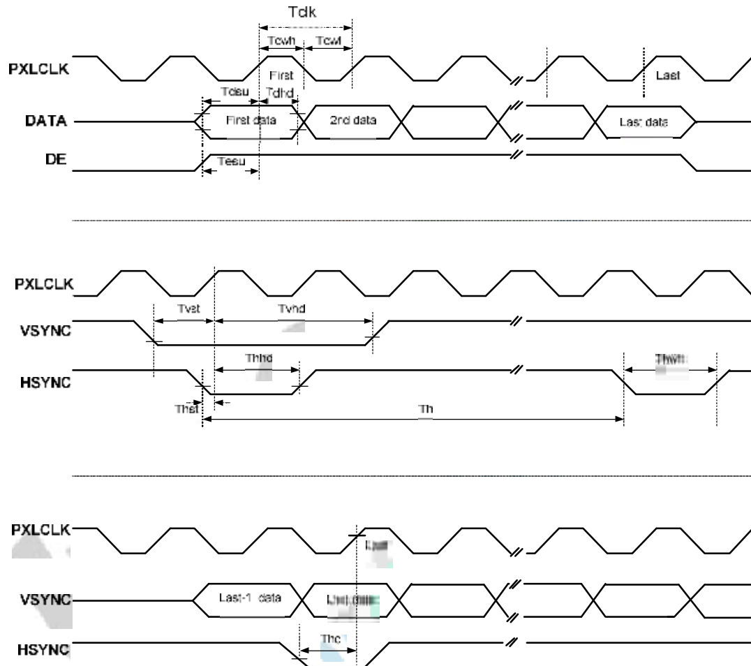
Fig.3-1 Clock and Data Input Timing Diagram
