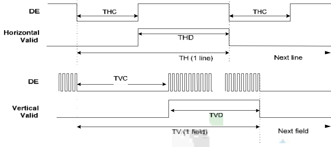
Fig.3-2 DE Mode Input Timing
