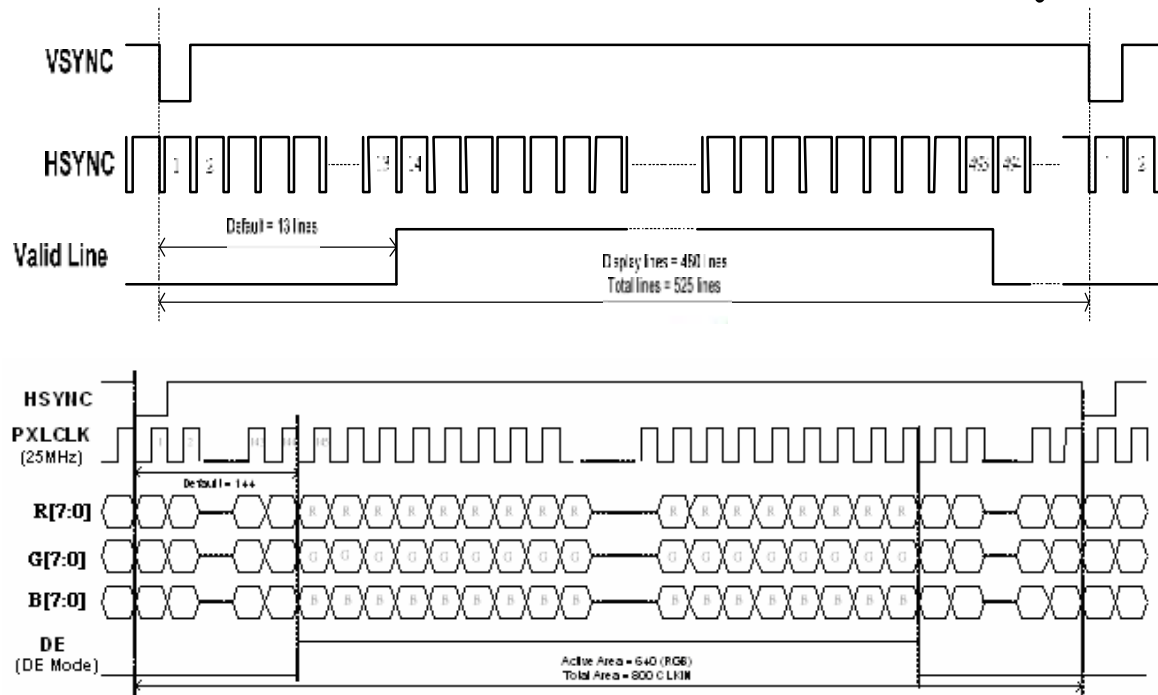
Fig. 3-4 24 bit RGB mode for 640 x (RGB) x 480
